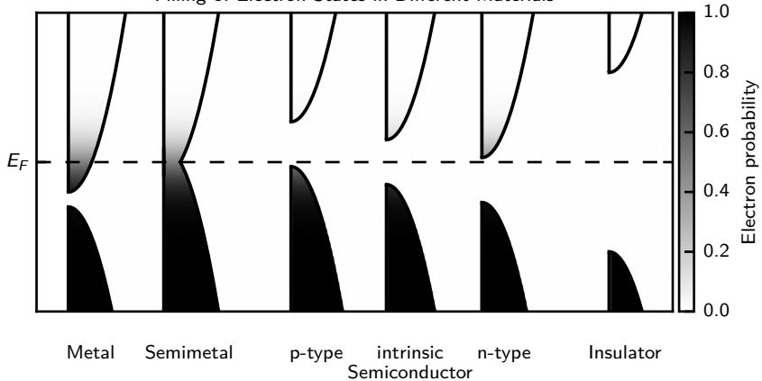
Filling of Electron States in Different Materials
